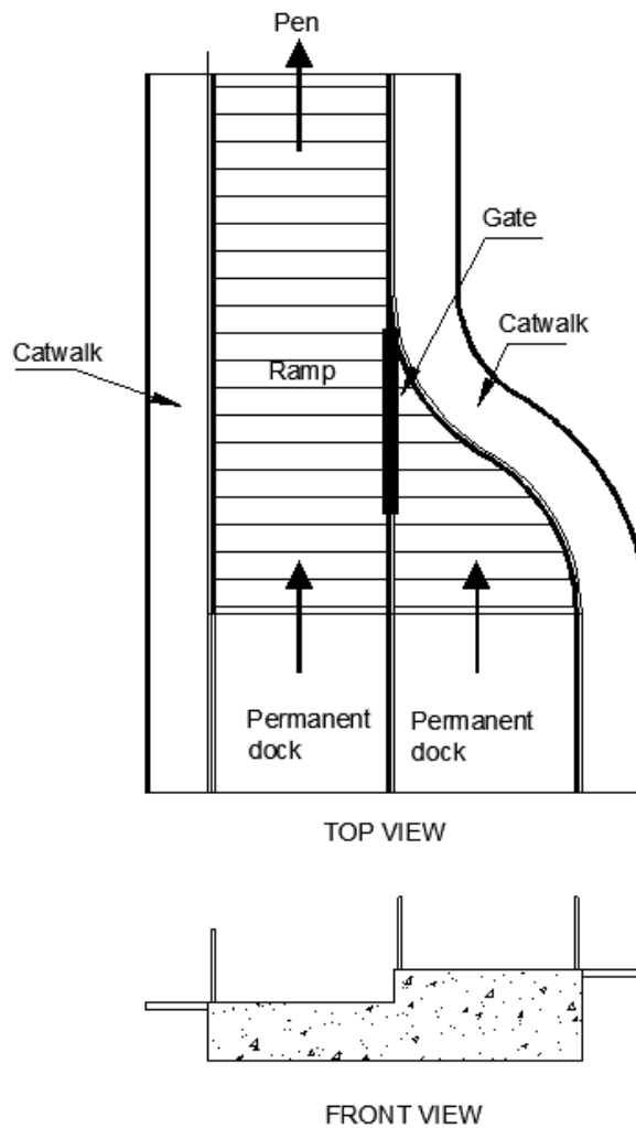
Figure 2 – Permanent multilayer dock with ramp
