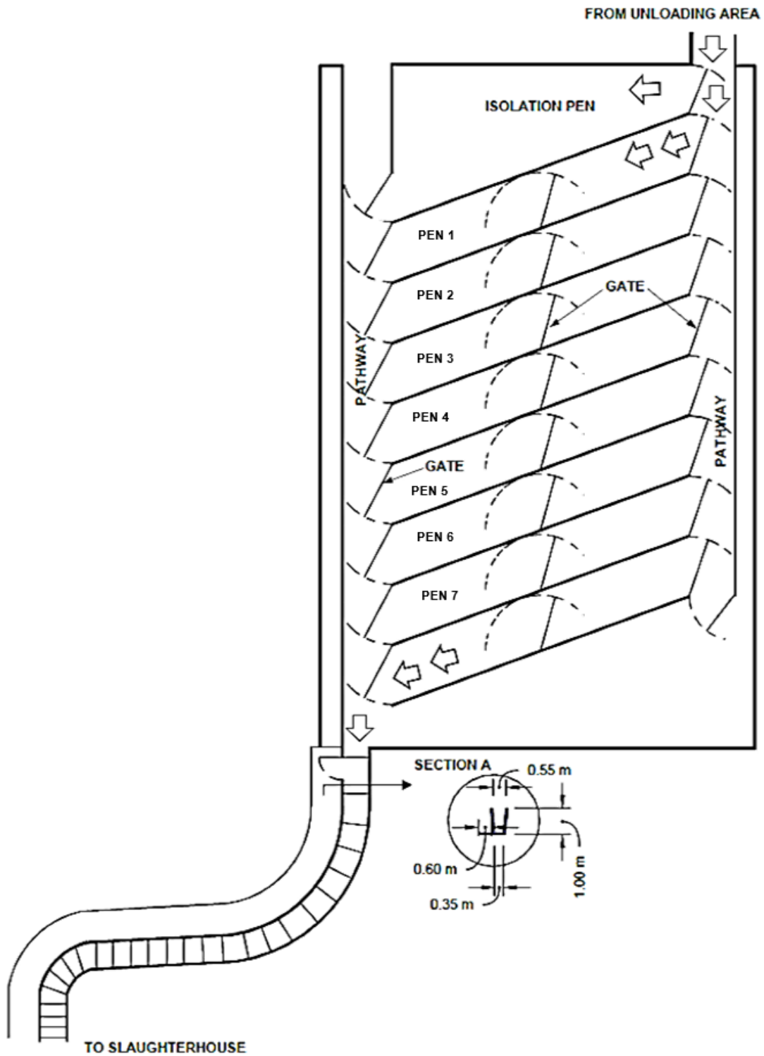
Figure A.1 – Sample of Elongated Lairage Layout Design for Swine
