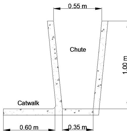
Figure 5 – Swine Chute
