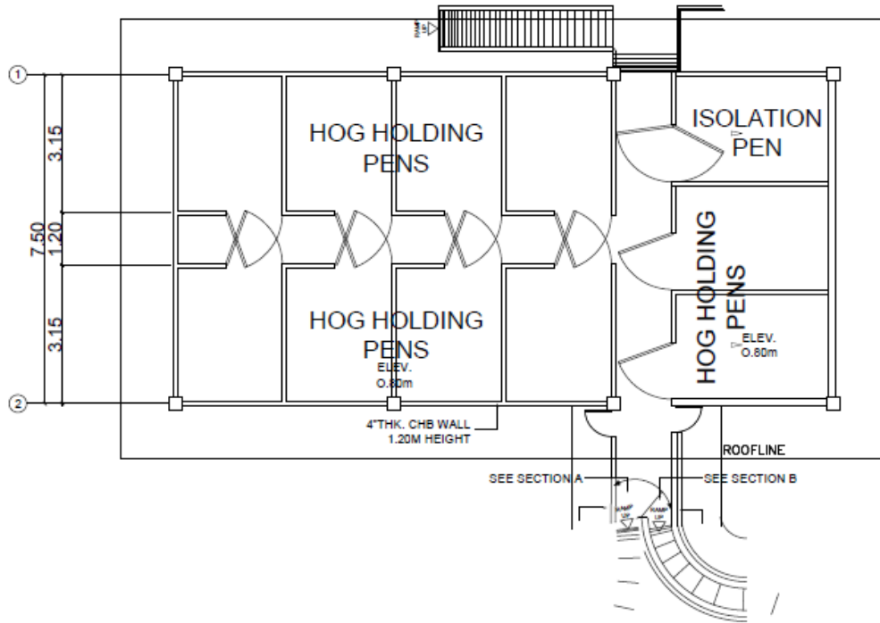
Figure A.1 – Sample of Typical Lairage Layout Design for Swine
