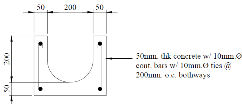
Figure 6– Swine Concrete Water trough
